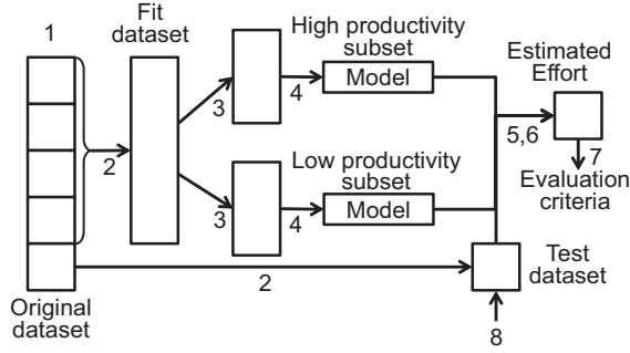
Figure 3. Experimental procedure (two-level model)
