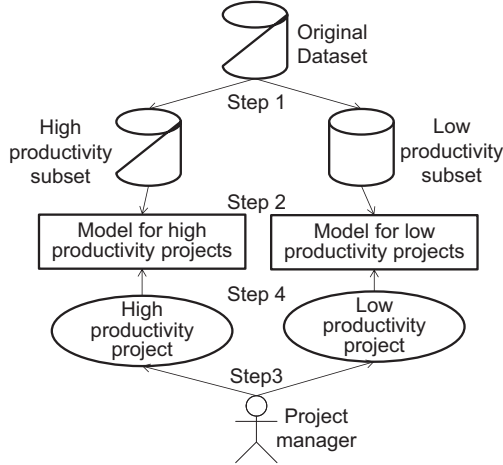
Figure 1. Procedure of the expert judgment incorporated estimation (two-level model)
