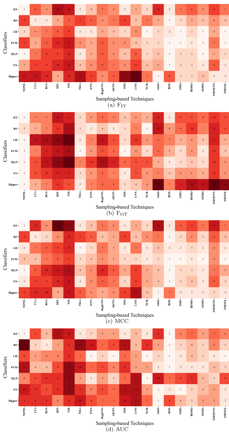
Fig. 3 The rank of SKESD test of each sampling-based technique for each classifier among all projects in terms of all four indicators
