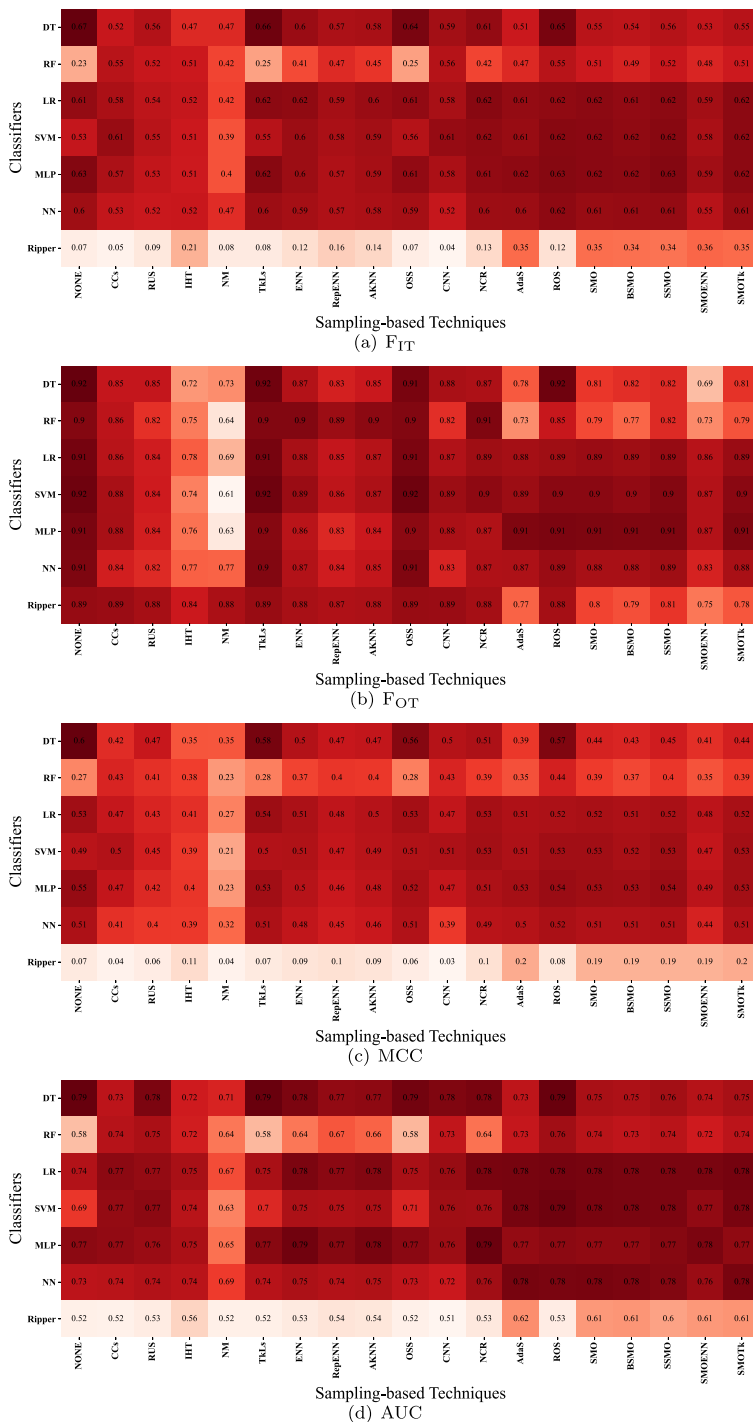
Fig. 2 Average value of each sampling-based technique for each classifier among all projects in terms of all four indicators
