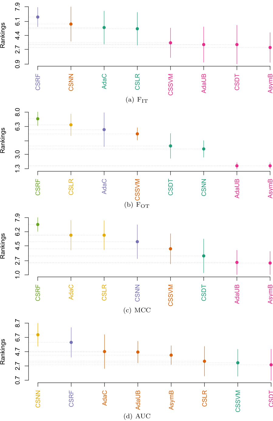
Fig. 7 SKESD rank of each cost-sensitive-based technique across all projects in terms of all four indicators
