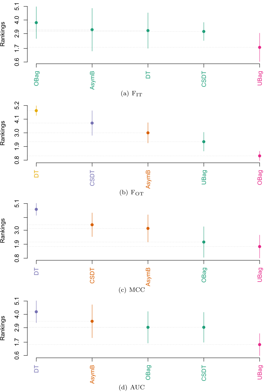
Fig. 8 SKESD rank of the five imbalanced learning techniques in cross-project scenario in terms of all four indicators
