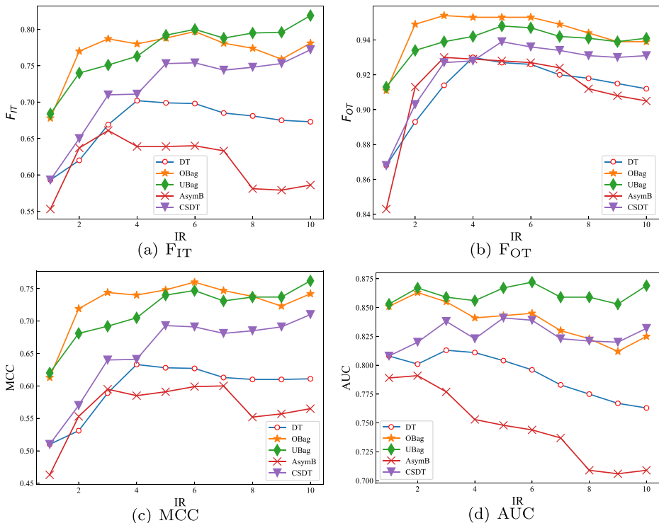
Fig. 9 Line chart of average value of the five imbalanced learning techniques under different imbalance levels in terms of all four indicators
