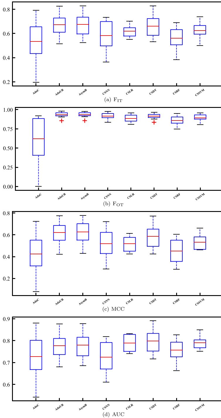
Fig. 6 Box plot of average value of each cost-sensitive-based technique among all projects in terms of all four indicators
