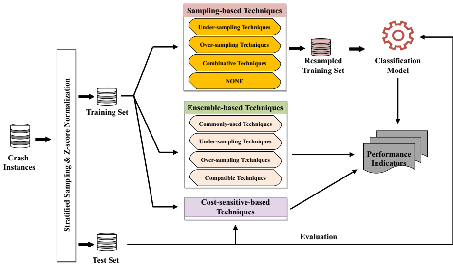
Fig. 1 An overall framework of our experiment process
