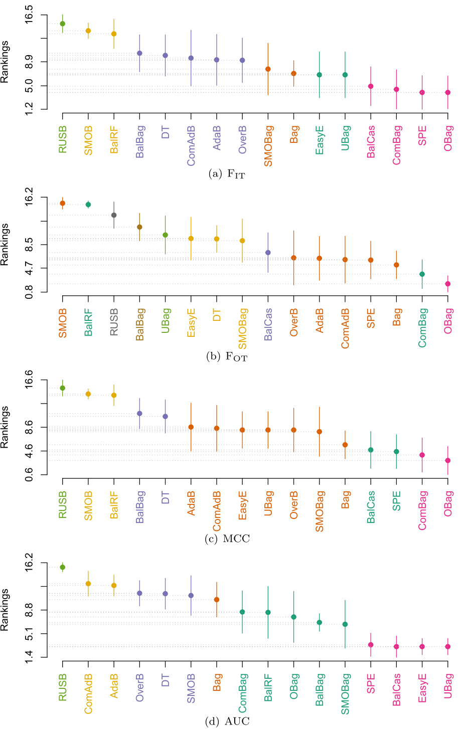
Fig. 5 SKESD rank of each ensemble-based technique across all projects in terms of all four indicators
