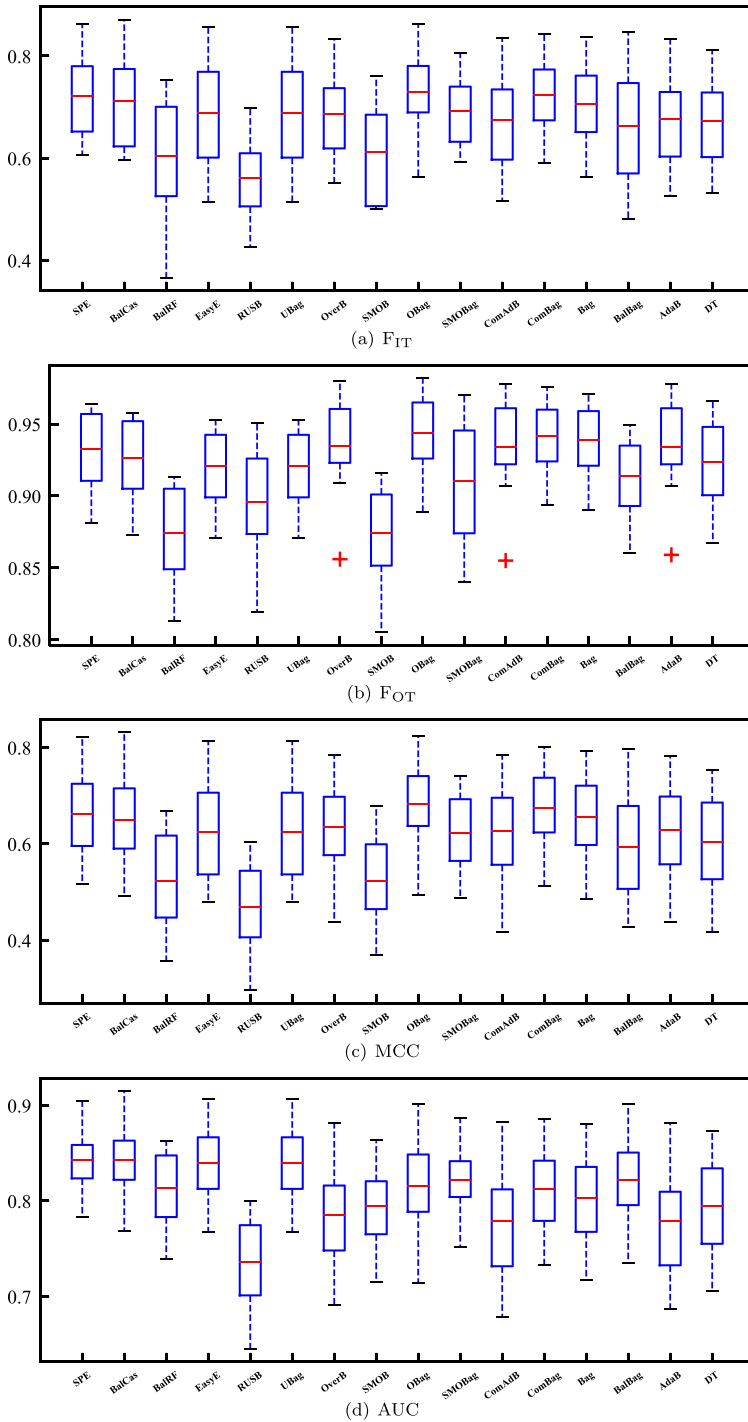
Fig. 4 Box plot of average value of each ensemble-based technique among all projects in terms of all four indicators
