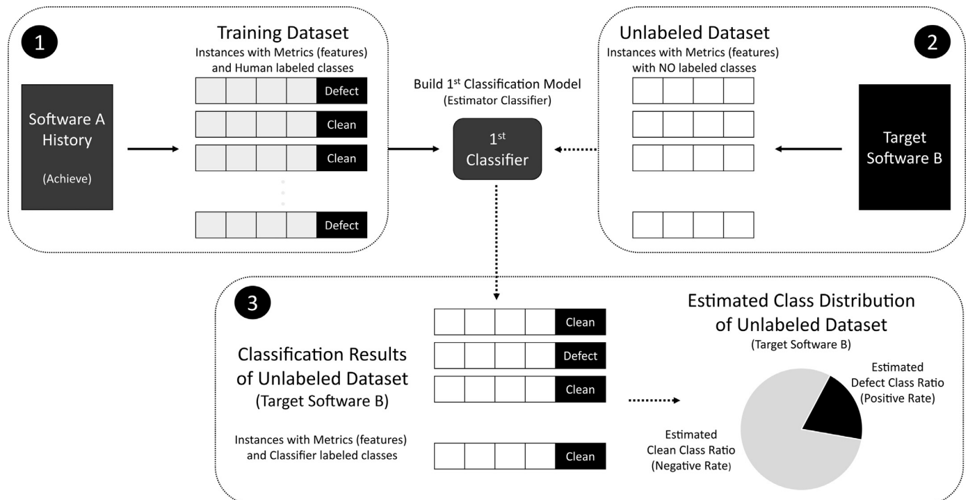
Fig. 2. CDE-SMOTE Diagram: Class Distribution Estimation.
