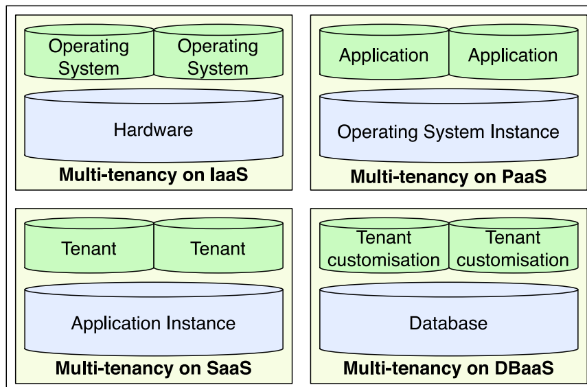
Fig. 5. Multi-tenancy on different service layers.
