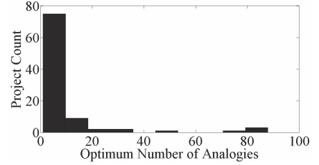
(b) Nasa93
